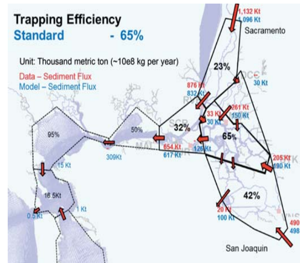
Bay Delta Community model by Deltares, developed in collaboration with USGS, SFEI, Berkeley etc.
