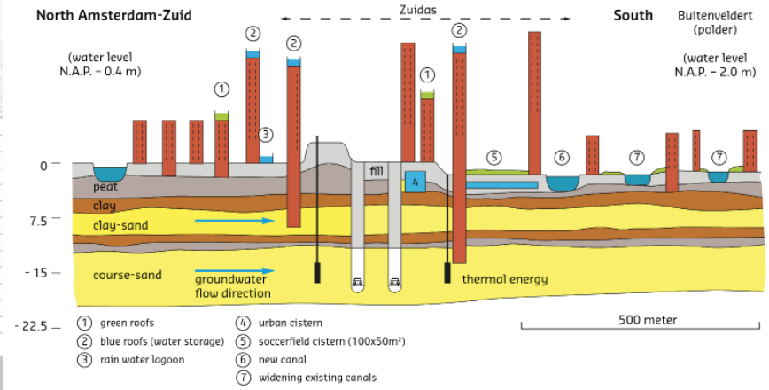
Zuidas, Amsterdam, water measures to enable functioning of new tunnels and overall water system
